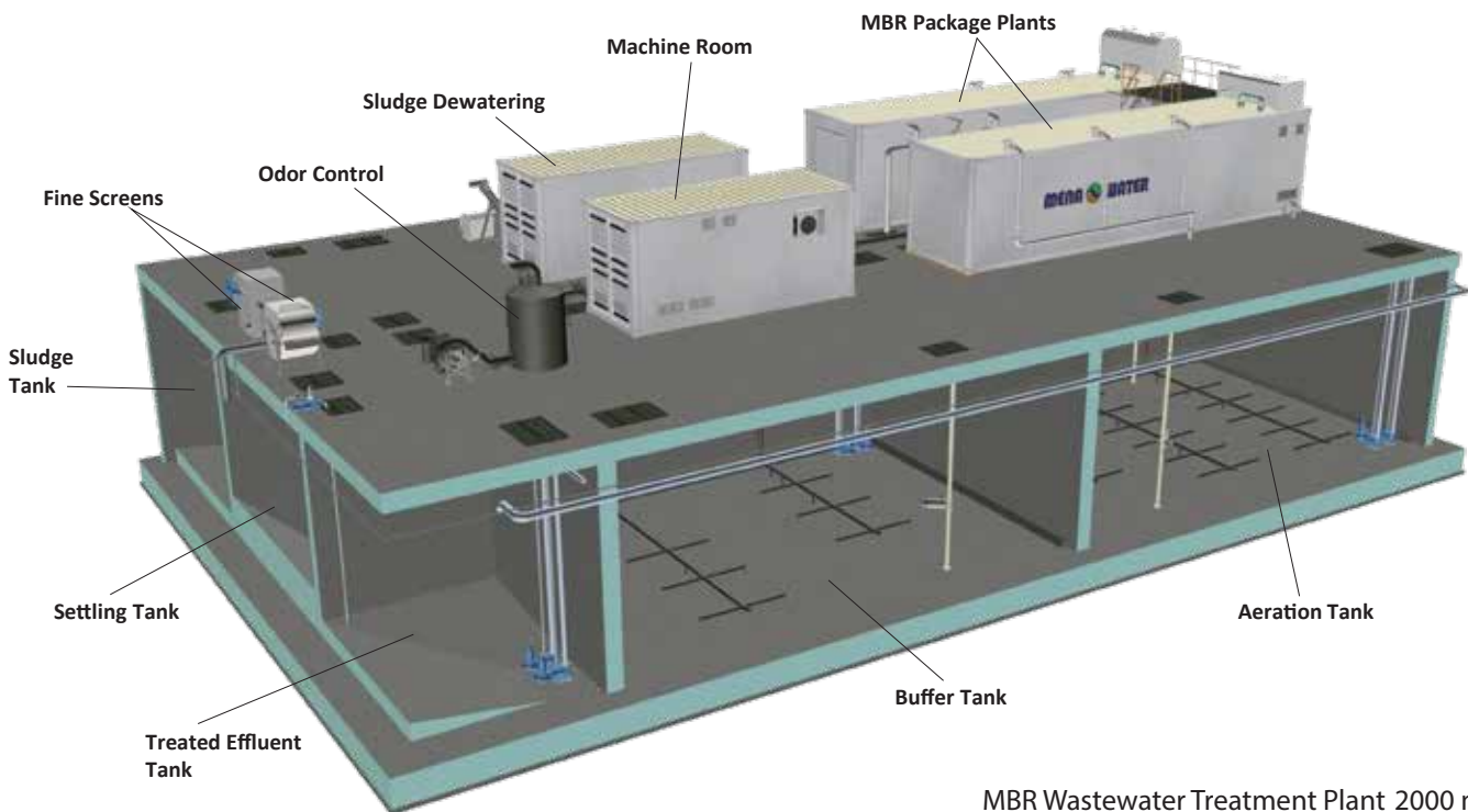
MBR Wastewater Treatment Plant 2000 m³/d
